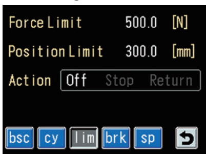
Limit settings
